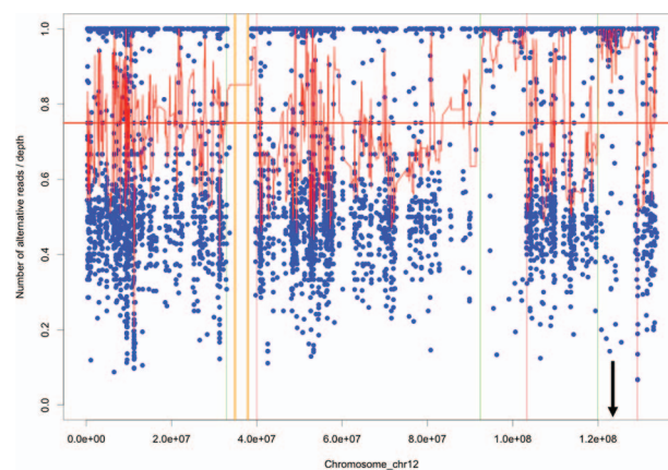
Supplementary Figure S2 Homozygosity stretch on chromosome 12 in GL-13. The stretch is located between chr12:119960612 and 129181719. The blue dots represent the variants, the vertical orange lines represent the centromere, the horizontal red line is a moving average of the mean frequency of the alternative allele of nearby variants, the vertical green and red lines represent the start and stop location of the homozygosity stretch and the black arrow represents the location of CCDC62 . The figure was made by RareVariantVis. Positions refer to genome build GRCh37/hg19.
