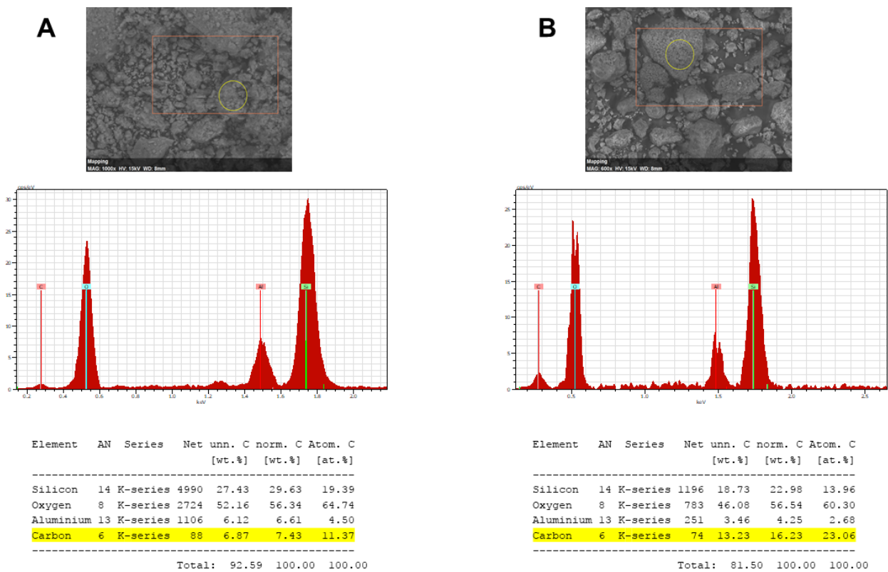
Figure S1: Raw data from EDX measurements of (A) CTS-zeolite and (B) CA-CTS-zeolite, including (from up to down): mapping window, EDX spectrum, table with element composition.
