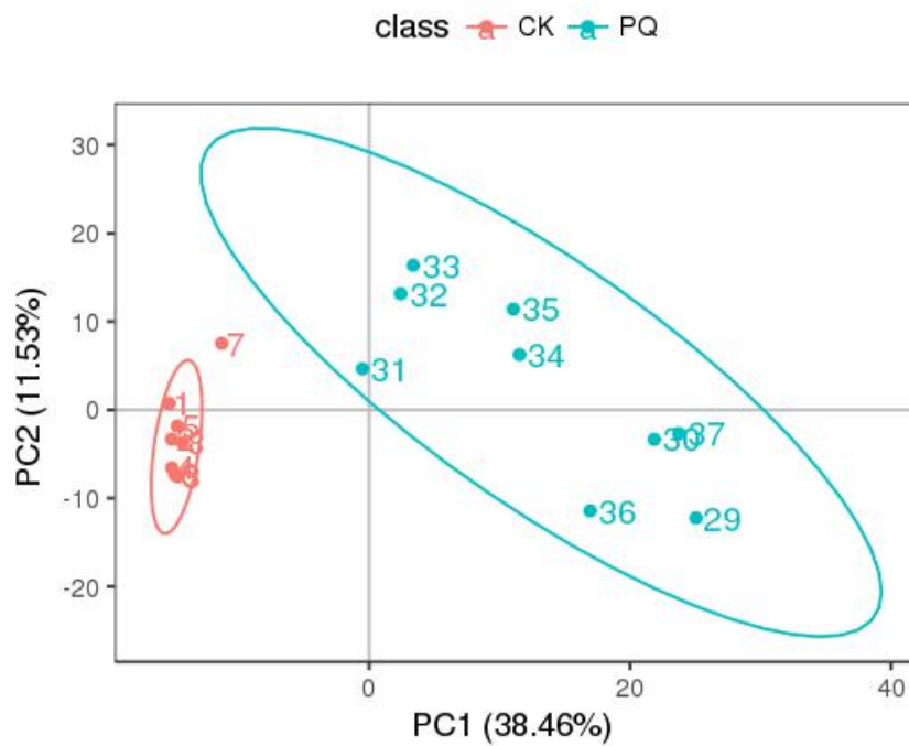
SI Fig.1. Principal component analysis between the PQ group and the control group, the upper figure was obtained in the negative mode, the bottom figure was obtained in the positive mode.
