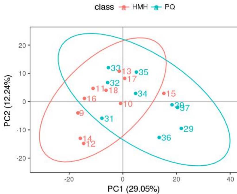
SI Fig.2. The principal component analysis between the HMH group and the PQ group (The upper figure was obtained in the negative polarity mode; the bottom figure was obtained in the positive polarity mode).
