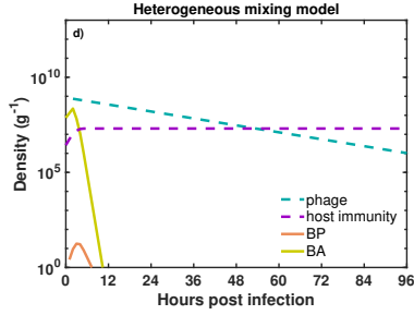
Combined therapy + Immune response against B_A inoculum
