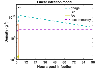
Combined therapy + Immune response against B_A inoculum
