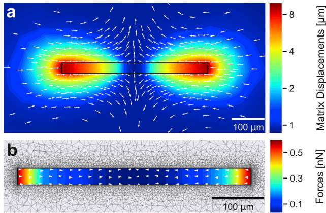
FIGURE 1 (a) Reconstructed matrix deformations (cross section through the z -plane) for a single contracting FDB fiber with a length of 446\ \mu\text{m} , a width of 32\ \mu\text{m} , and 4% strain. Displacement magnitude and direction are indicated by the colorbar and arrows. (b) Shown are reconstructed forces at the fiber surface. Absolute forces decrease toward the center. Total contractility is determined from the forces in the x -direction summed over all surface nodes from one end of the fiber to its center. The force direction is predominantly aligned along the fiber axis as indicated by arrows. An outward normal directed force component due to volume conservation becomes visible for small displacements near the center. To see this figure in color, go online.
