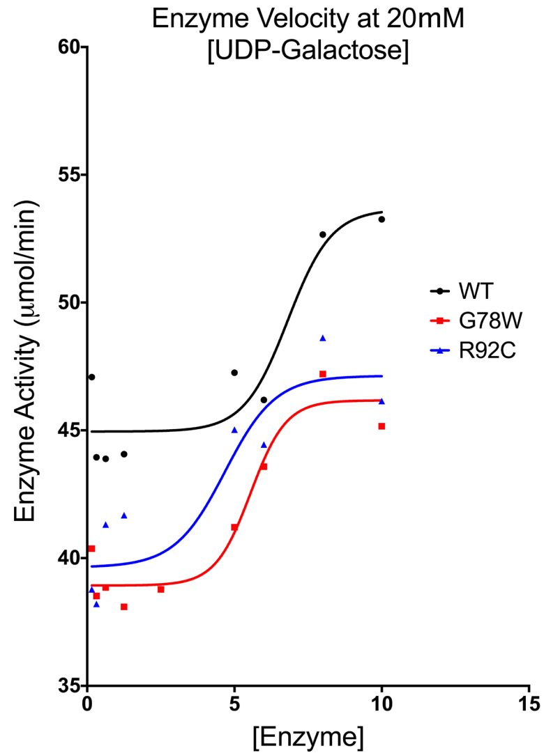
Figure S3: Enzyme velocity at fixed substrate concentration (20mmol/l) with variable enzyme concentration. GLT8D1-R92C and GLT8D1-G78W enzyme velocity is reduced compared to wild type at every enzyme concentration, indicating lower enzyme activity. Related to Figure 4.
