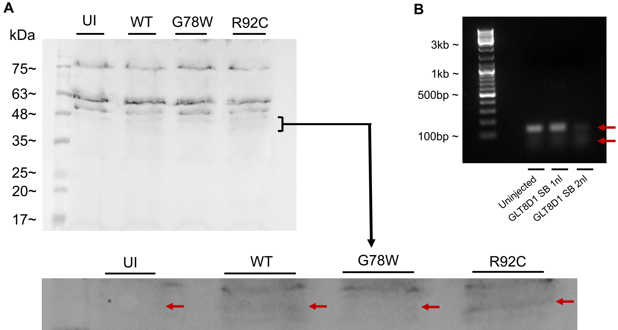
Figure S2: Knockdown and overexpression of mutant and WT GLT8D1 in vivo . Overexpression of GLT8D1-R92C mutant and WT GLT8D1 in zebrafish embryos ( A ); band at ~44kDa, equivalent to the predicted size of GLT8D1, is present in all overexpression conditions but not in uninjected zebrafish (arrowed); related to Figure 3B-D. GLT8D1 splice blocking (SB) morpholino successfully reduces expression of glt8d1 mRNA in zebrafish embryos ( B ); morpholino ~15ng/nll; F: ACTGGGATTGTTGATGTTGAG, R:TAACCACATTCACTCTGCGT, predicted size 133bp; related to Figure 3A.
