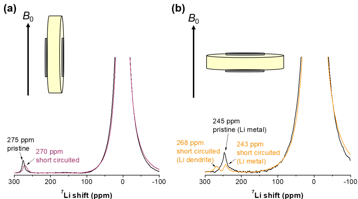
Figure S6. ^7\text{Li} NMR of pristine (black) and short circuited (purple in (a) and orange in (b)) Li-LLZTO-Li symmetrical cells with the electrodes oriented (a) parallel and (b) perpendicular to B_0 .
