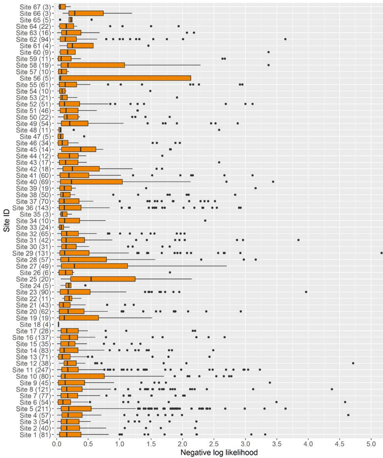
Figure S9.2 Performance by clinical site of the CDP model. Prediction performance of the CDP model for all clinical sites, measured by the negative log-likelihood. For every site, a boxplot of negative log-likelihoods for the patients being part of the site is shown. Numbers in brackets indicate the number of patients for a given clinical site.
