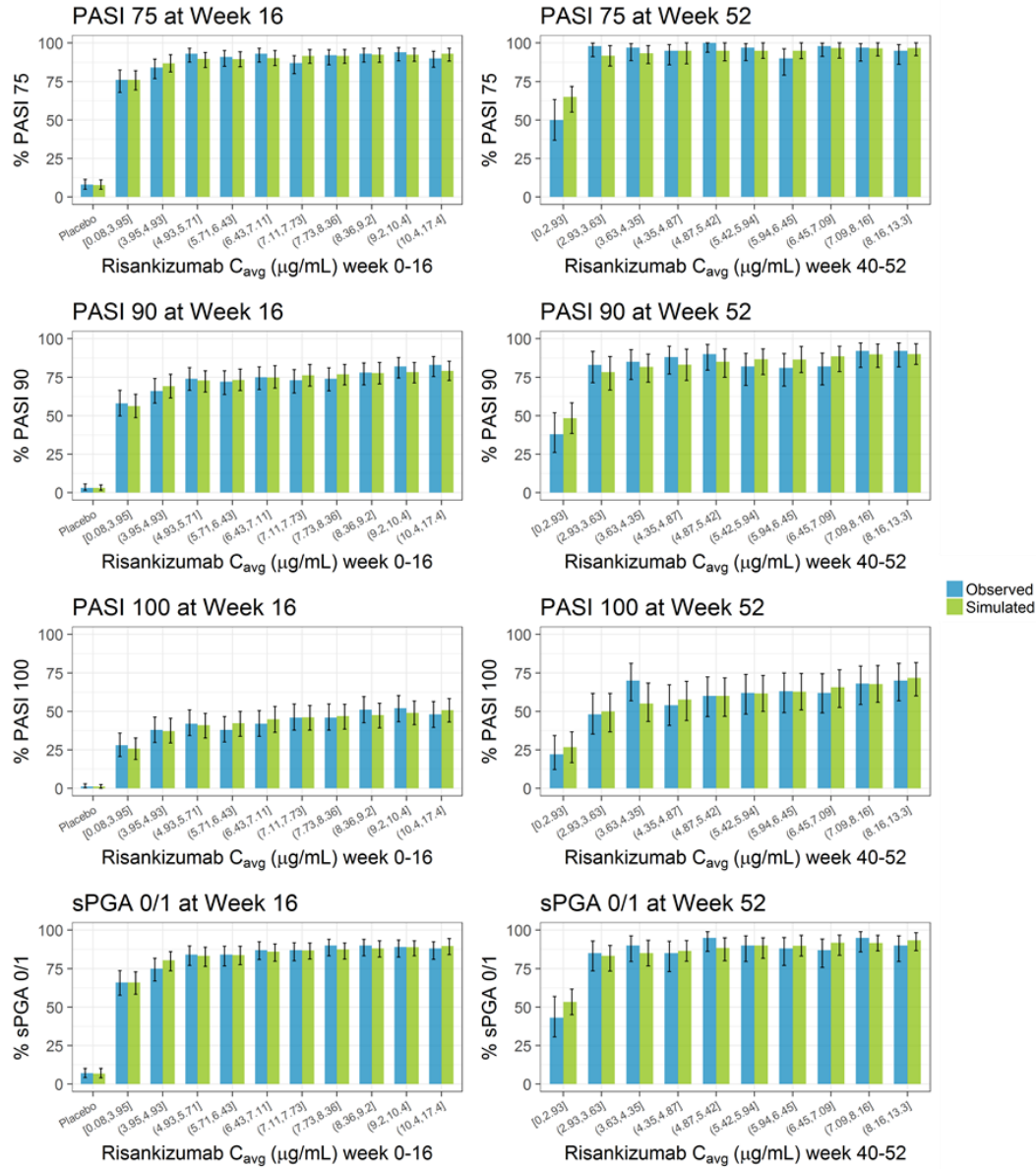
Figure S2. Graphical comparison of observed and model-predicted probability of PASI and sPGA endpoints at weeks 16 and 52 based on analyses of the Phase 2 and 3 trials
