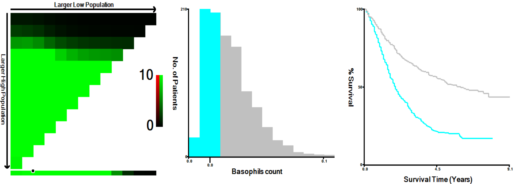
Figure S2. X-tile analyses of DFS was performed to determine the optimal cut-off values for basophils count.
