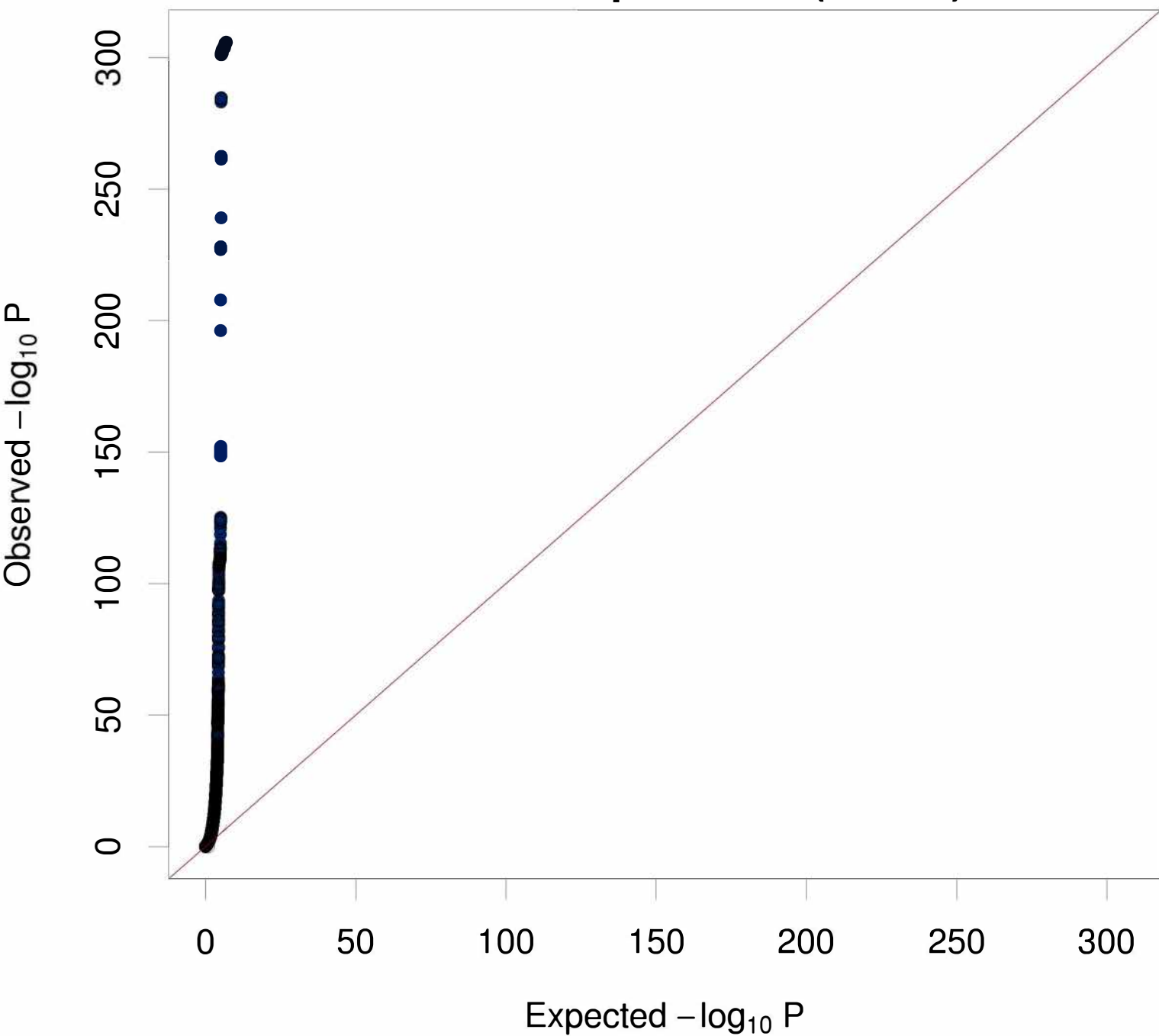
Figure S12. QQ-plot of BMI Lambda GC: 2.566 LDSC intercept: 1.1234 (0.0297)
