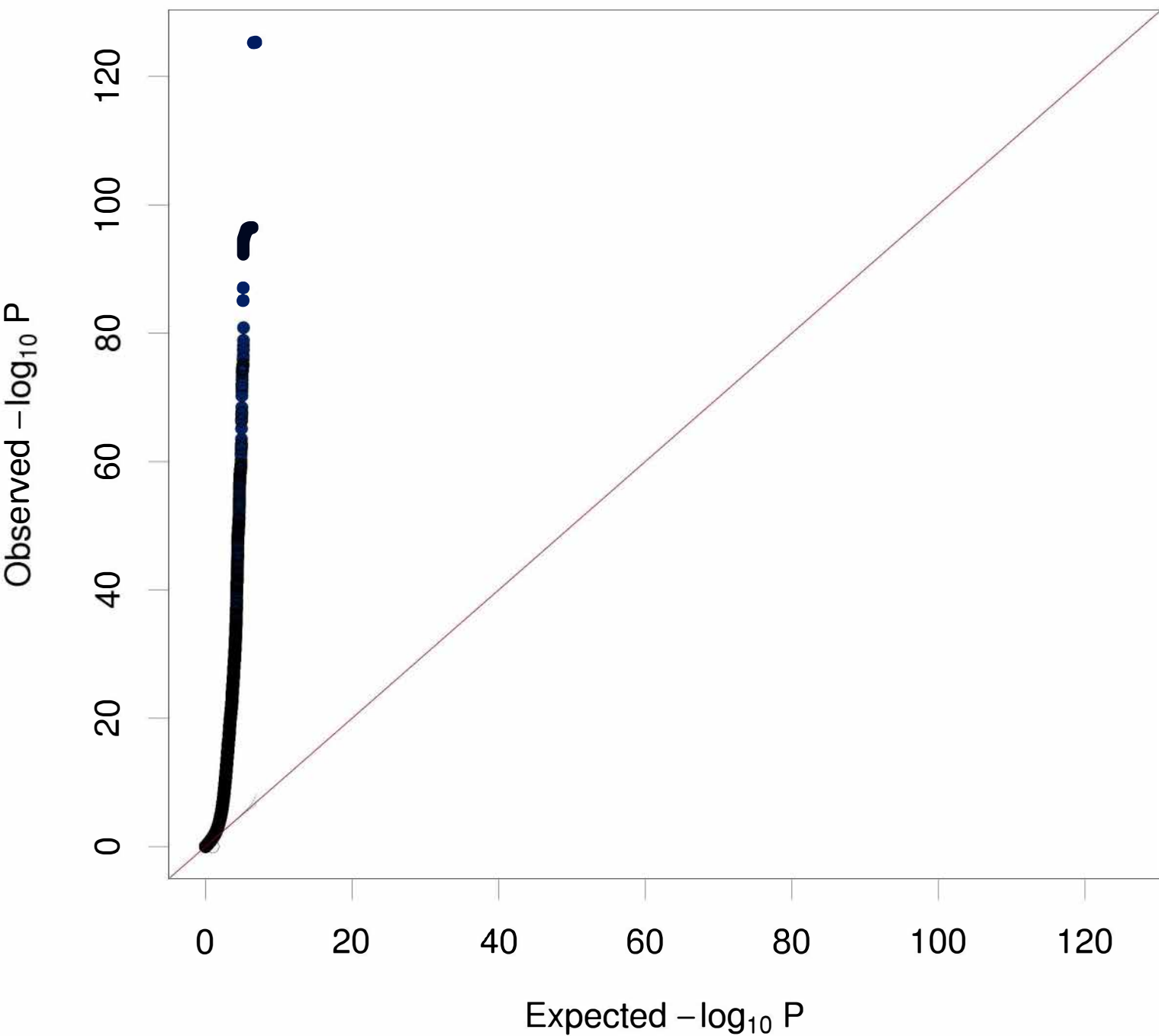
Figure S14. QQ-plot of waist circumference adjusted by BMI Lambda GC: 1.842 LDSC intercept: 1.1708 (0.0334)
