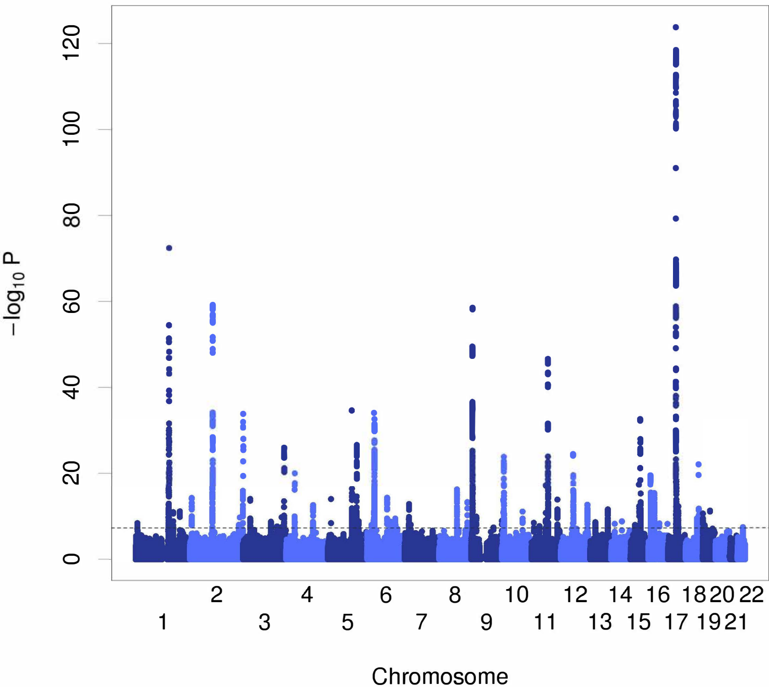
Figure S2. Manhattan plot of early-onset asthma
