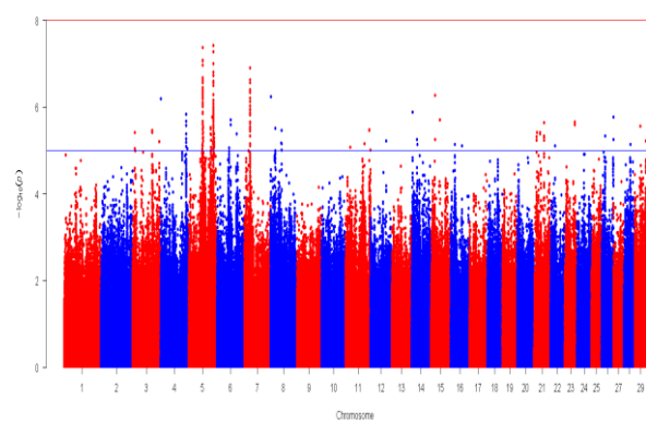
Figure S2: Manhattan plots for wither height in a) Angus, b) Charolais, c) Hereford, d) Limousin, e) Simmental, and f) stature in Holstein-Friesian.
