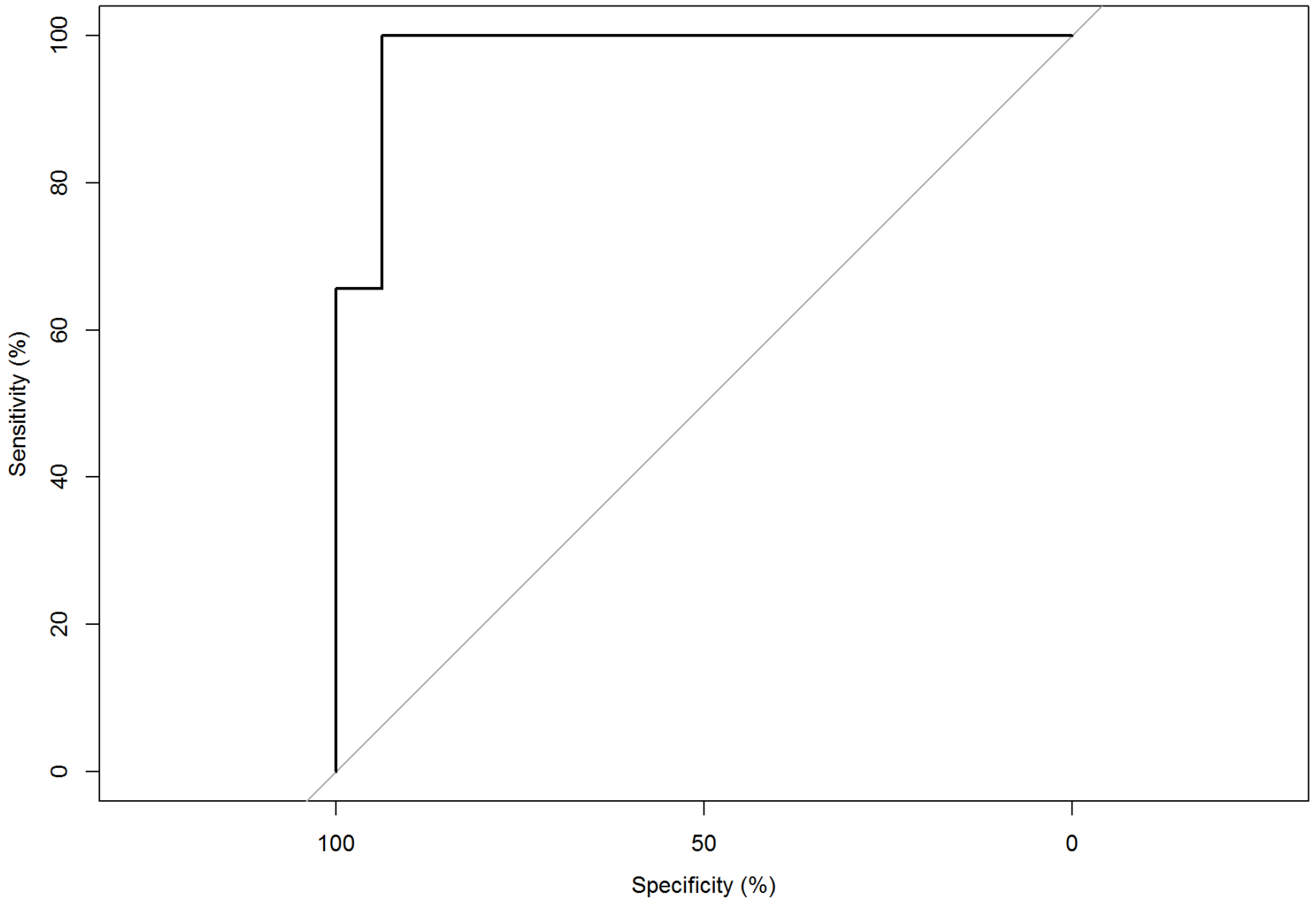
S2 Figure. ROC curve of normalized tibial translation ( \Delta_N ) considering Group PA (pathological stifles) and Group CO (contralateral stifles).
