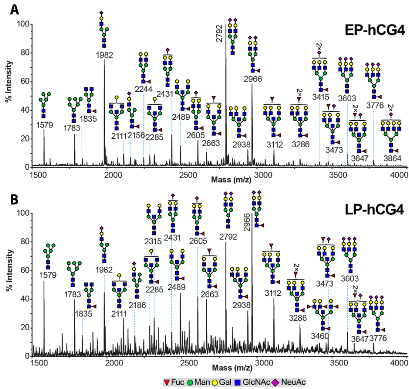
S6 Fig. N-glycomic profiles of pre-eclampsia samples. MALDI-TOF MS spectra of permethylated N-glycans derived from (A) EP-hCG4 and (B) LP-hCG4 samples. Putative structures are based on composition, tandem MS. All molecular ions are [M+Na]^+ .
