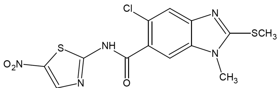
Compound CMC-20 : 5-chloro-1-methyl-2-(methylsulfanyl)- N -(5-nitro-1,3-thiazol-2-yl)-1 H -benzimidazole-6-carboxamide.
