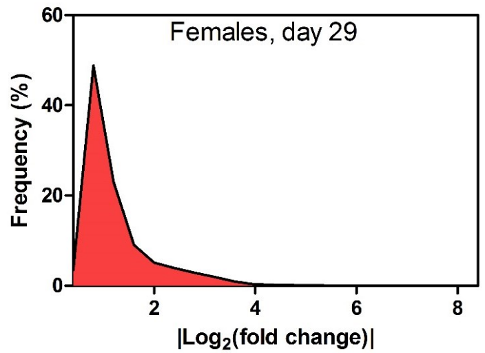
Figure S1. Frequency distribution of absolute fold changes of genes differentially expressed ( |\text{fold change}| \geq 1.5 & \text{FDR} \leq 0.05 ) in Wistar rats gavaged daily with acetamide. Fold changes from the highest dose group (1500 mkd) was used to calculate frequency, expressed as percent of DEGs.
