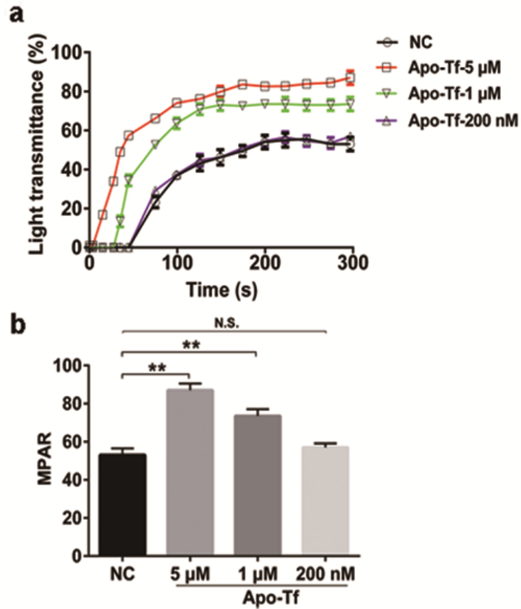
Fig. S6 Effects of apo-transferrin on thrombin-induced platelet aggregation.
