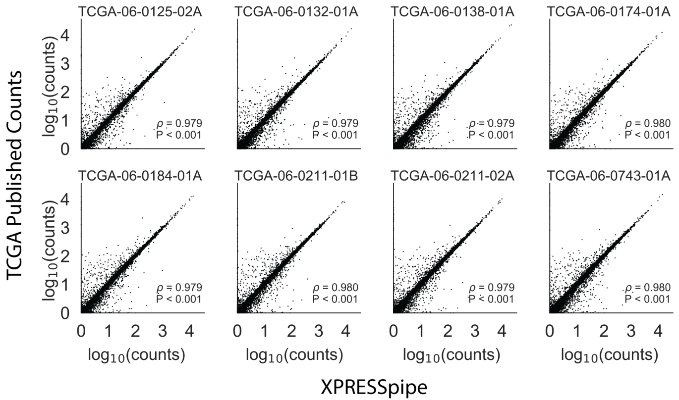
Fig. A. Pipeline validation using publicly available TCGA count data. Correlations were calculated between publicly available count data from TCGA samples and the count data processed by XPRESSpipe. Pseudogenes were excluded from the analysis. All reported \rho values are Spearman correlation coefficients. XPRESSpipe-processed read alignments were quantified to Homo sapiens build CRCh38v98 using an unmodified GTF.
