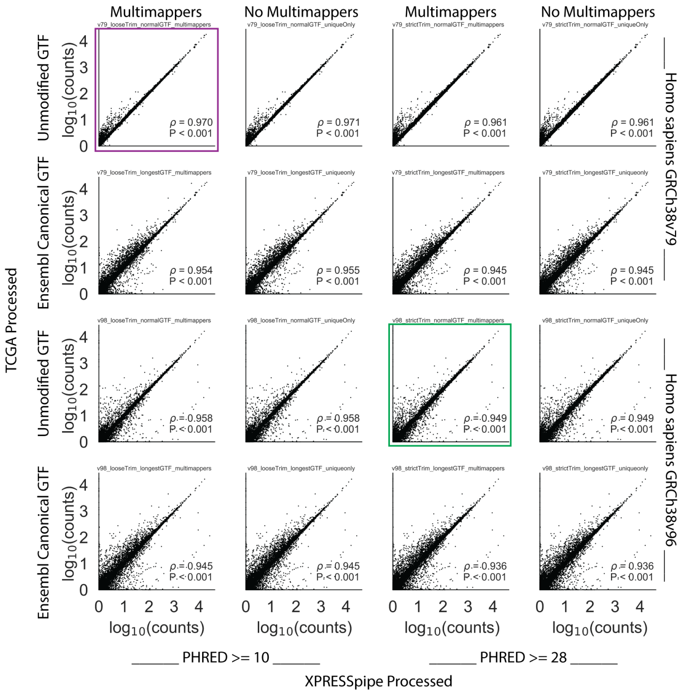
Fig. B. Sample RNA-Seq count data compared between TCGA count data and various conformations of the XPRESSpipe pipeline. An overview of how different conformations of the XPRESSpipe perRNAseq pipeline compared to the published TCGA sample TCGA-06-0132-01A count data. The x-axis data for the plot enclosed in maroon most closely mirrors the settings used in the published TCGA RNA-Seq pipeline. The x-axis data for the plot enclosed in green used XPRESSpipe default settings and the most current reference transcriptome at the time of writing. All \rho values reported are Spearman correlation coefficients.
