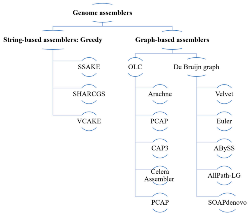
Figure S1. Summary of the tree main genome assemblers' methods and the most widely used software that applies each method.
