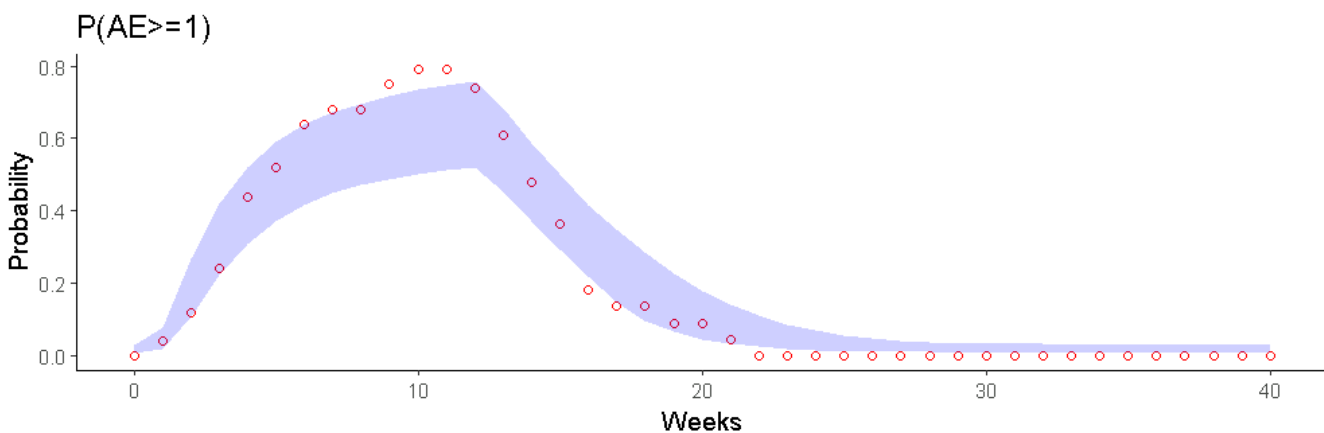
Figure S7: The simulation for the PK profiles of unbound vismodegib in the plasma and effect compartment and the proportion of grade \geq 1 muscle spasm was based on 150mg daily dose for 12-weeks with 24-weeks washout using the PO model. The actual age and body weight (from the 74 patients in the dataset), and the typical value of AAG ( 30 \mu\text{M} ) were used in the simulation as PK covariate. 500 simulations with 200 patients for each simulation (sampling with replacement from the 74 patients) were conducted. The shaded areas are the 95% prediction intervals. The observed proportion of grade \geq 1 muscle spasm over time (red cycle) was from the cohort 2.
