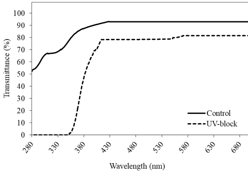
Supplementary Figure S1. Transmission spectra of UV-transmitting filter (Control, black line) and UV-blocking filter (UV-block, dashed line) used to cover the tunnels under field conditions.
