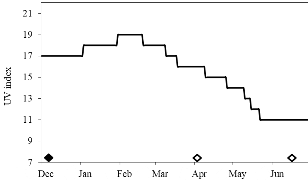
Supplementary Figure S2. Maximum daily erythemal UV index at the experimental site (Junín, Peru). Data were collected between December 2016 and June 2017. Sowing (closed diamonds) and sampling dates (open diamonds) are indicated at the bottom of the graph. For details, see Material and Methods.
