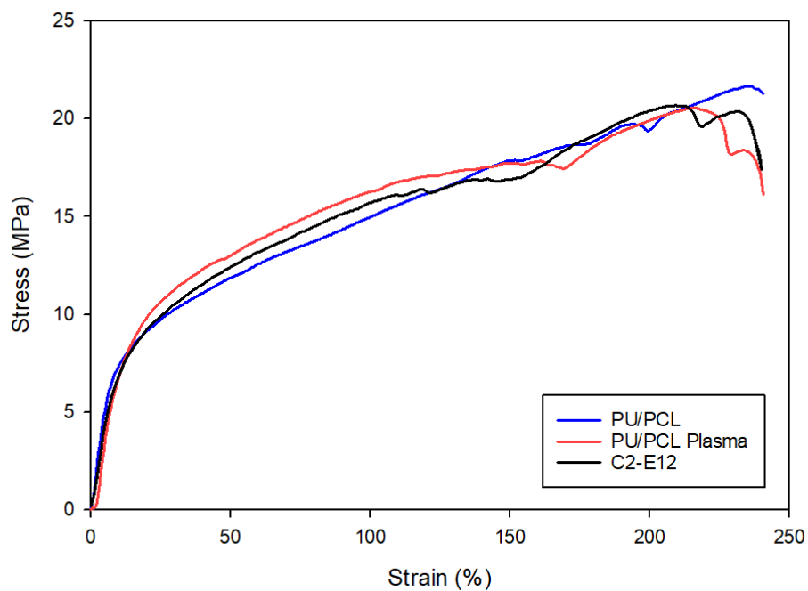
Figure S1. Stress-strain curve of the membranes when subjected to tension.
