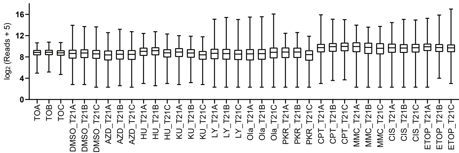
Boxplot for reads distribution
