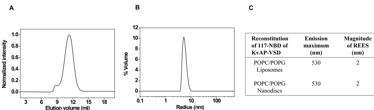
FIGURE S1 Fluorescence properties of 117-NBD mutant of KvAP-VSD in liposomes and Nanodiscs. (A) Gel filtration profile shows the efficient Nanodiscs assembly of the NBD-labeled KvAP mutant. (B) Volume-weighted particle size distribution of Nanodiscs obtained by DLS. The hydrodynamic diameter of Nanodiscs is found to be ~12 nm, which is in good agreement with previous studies (S2). (C) Comparison of fluorescence properties such as emission maximum and REES is shown for 117-NBD mutant of the sensor reconstituted in PC/PG liposomes and Nanodiscs. Interestingly, the identical values of fluorescence parameters in liposomes and Nanodiscs probably suggest negligible curvature effects on the structural dynamics of the sensor in membranes. See Materials and Methods for other details.
