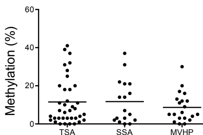
(E) IGFBP7
