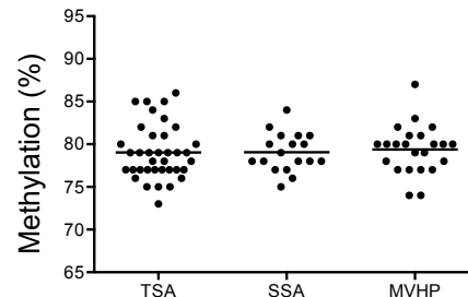
(I) LINE-1
