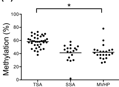
(H) SOX5
