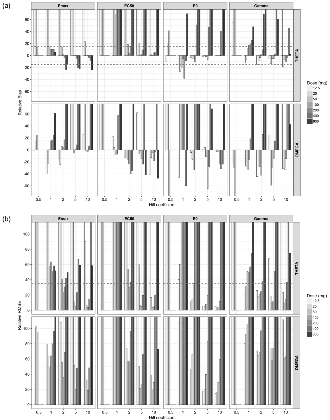
Supplementary Figure 1. Relative bias (a) and relative root mean square error (b) of pharmacodynamic parameters estimates for the multiple-dose scenarios.
