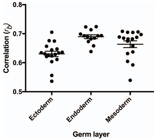
Supplementary Figure S4 Correlation of effects in germ layers. Correlation of cis-effects ( r_D ) between endometrium and 49 tissues grouped into germ layers from which they developed.
