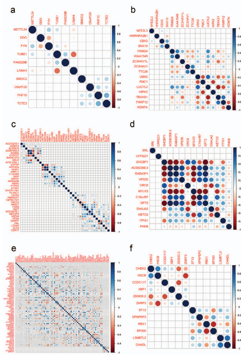
Supplementary Figure S6 Correlation between significant TWAS genes. Correlation plots showing the Pearson correlation between the predicted expression of genes at loci significantly associated with endometriosis in the TWAS analysis on chromosomes 6 (a), 7(b), 12(c), 16(d), 17(e) and 22(f).
