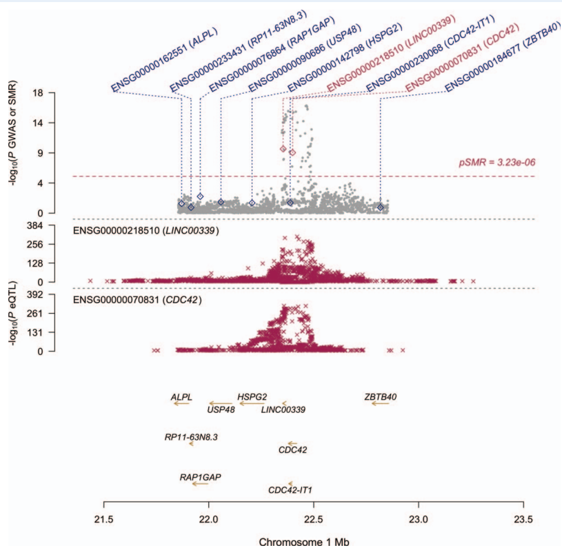
Supplementary Figure S7 SMR locus plot of the CDC42/LINC00339 locus. In the top plot, grey dots represent P-values for SNPs reported in Sapkota et al.'s (2017) GWAS meta-analysis for endometriosis and diamonds represent the P-values for probes from the multi-SNP-based SMR test. Crosses in the middle and bottom plots represent the eQTL P-values of SNPs associated with expression of LINC00339 and CDC42 in blood respectively. Positions are in hg19.
