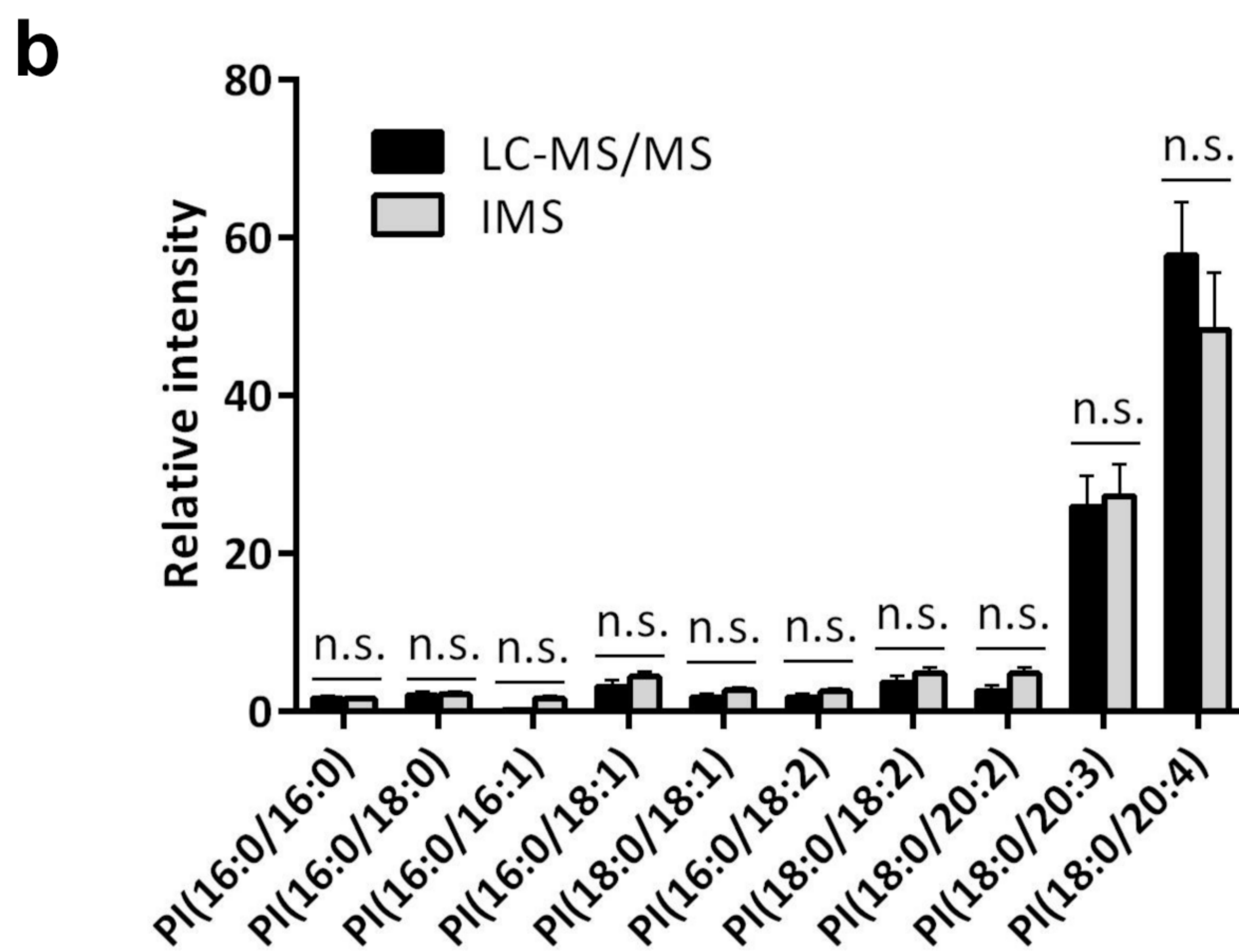
a. histological mapping of PIs in the breast tumor obtained from the patient derived xenograft. Blue line in bright view indicates the border of cancer cell cluster and surrounding stroma. Relative intensity of ion signals is represented by an RGB scale. Scale bar (white): 100 \mu m. b. Comparison between MALDI-IMS and Liquid chromatography (LC)-MS analysis of the same PDX-derived tumor. Two-way ANOVA with Sidak's post hoc multiple comparisons test. Error bar: SD.
