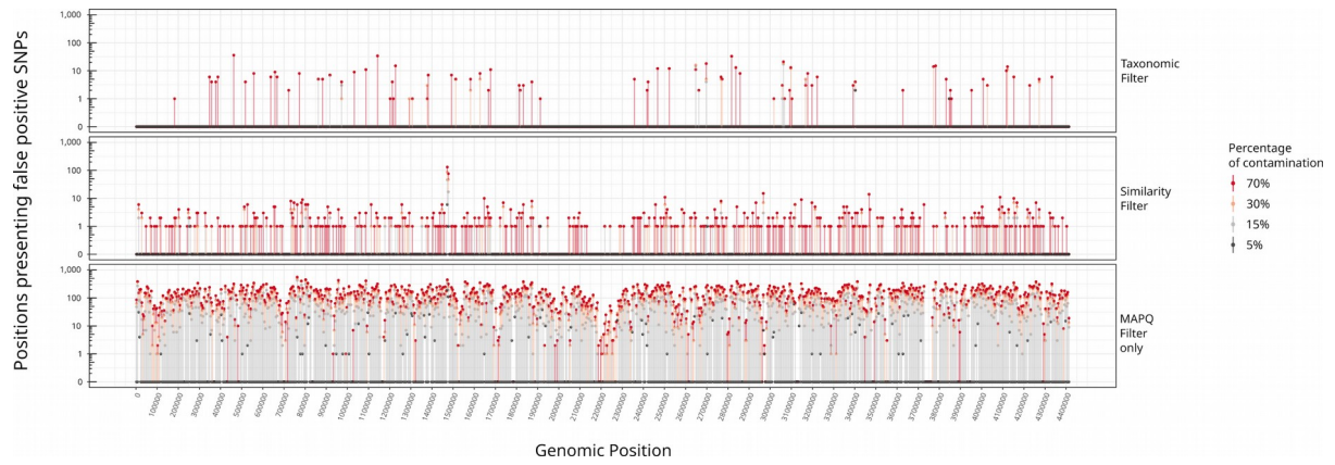
Figure S2. Contaminations can lead to incorrect calls across the M. tuberculosis genome. Number of positions (in 1,000 bp windows) with false positive SNPs arising from 5%, 15%, 30% and 70% contaminations with different organisms in mock contaminated MTB WGS samples.
