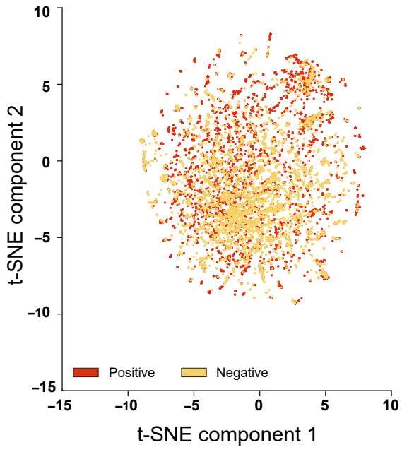
A Original input features
