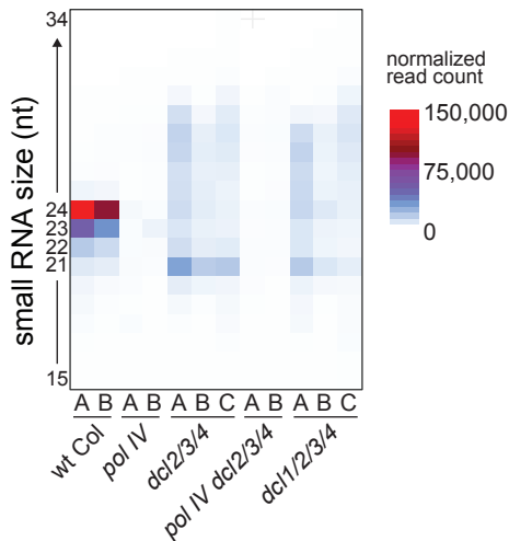
B Pol IV 21-22 nt sRNA clusters
