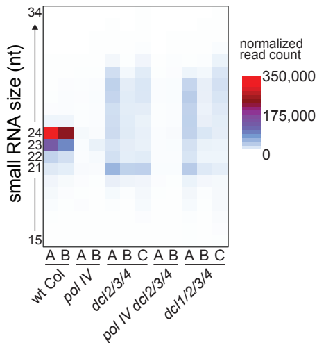
A Pol IV 24 nt siRNA clusters
