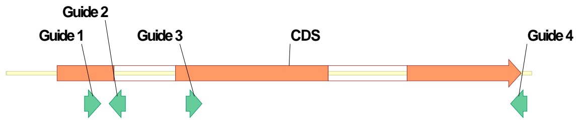
TaRPG1-A partial genomic region 745 bp
