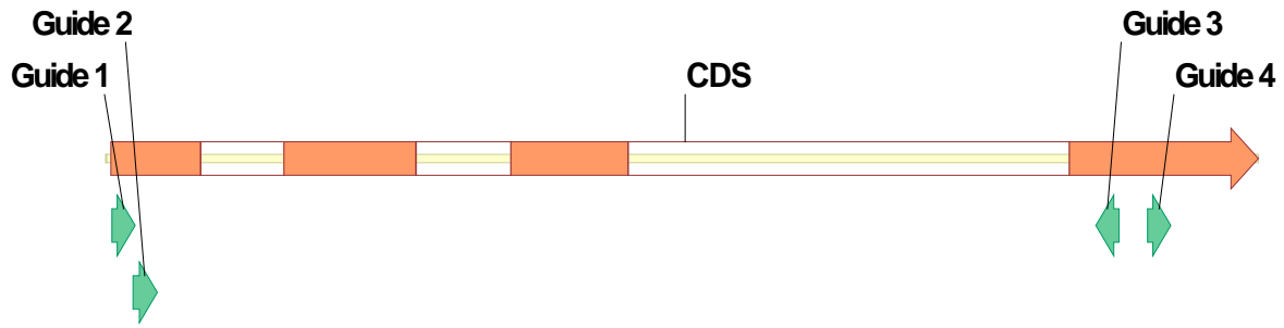
TaCaIS5-A partial genomic region 1125bp
