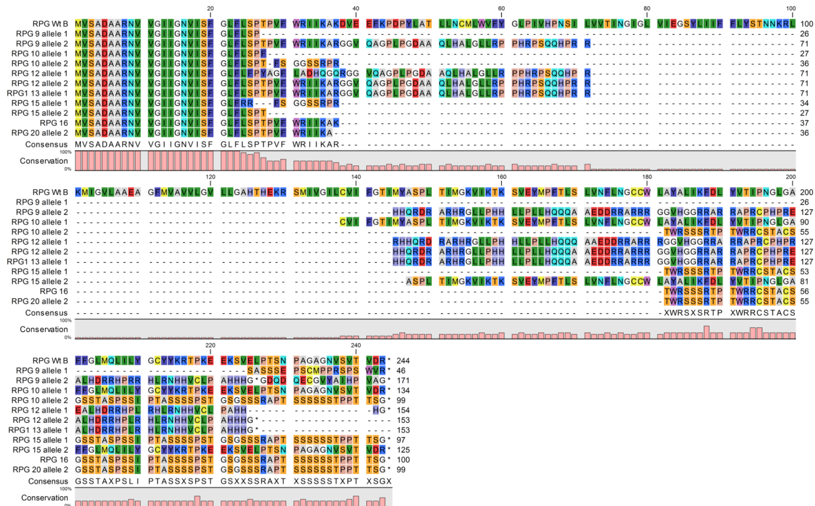
Suppl. Figure 7: Predicted amino acid consequences of the CRISPR Cas9 mutations in the TaRPG1-B homoeologue of all of the sterile plants produced.
