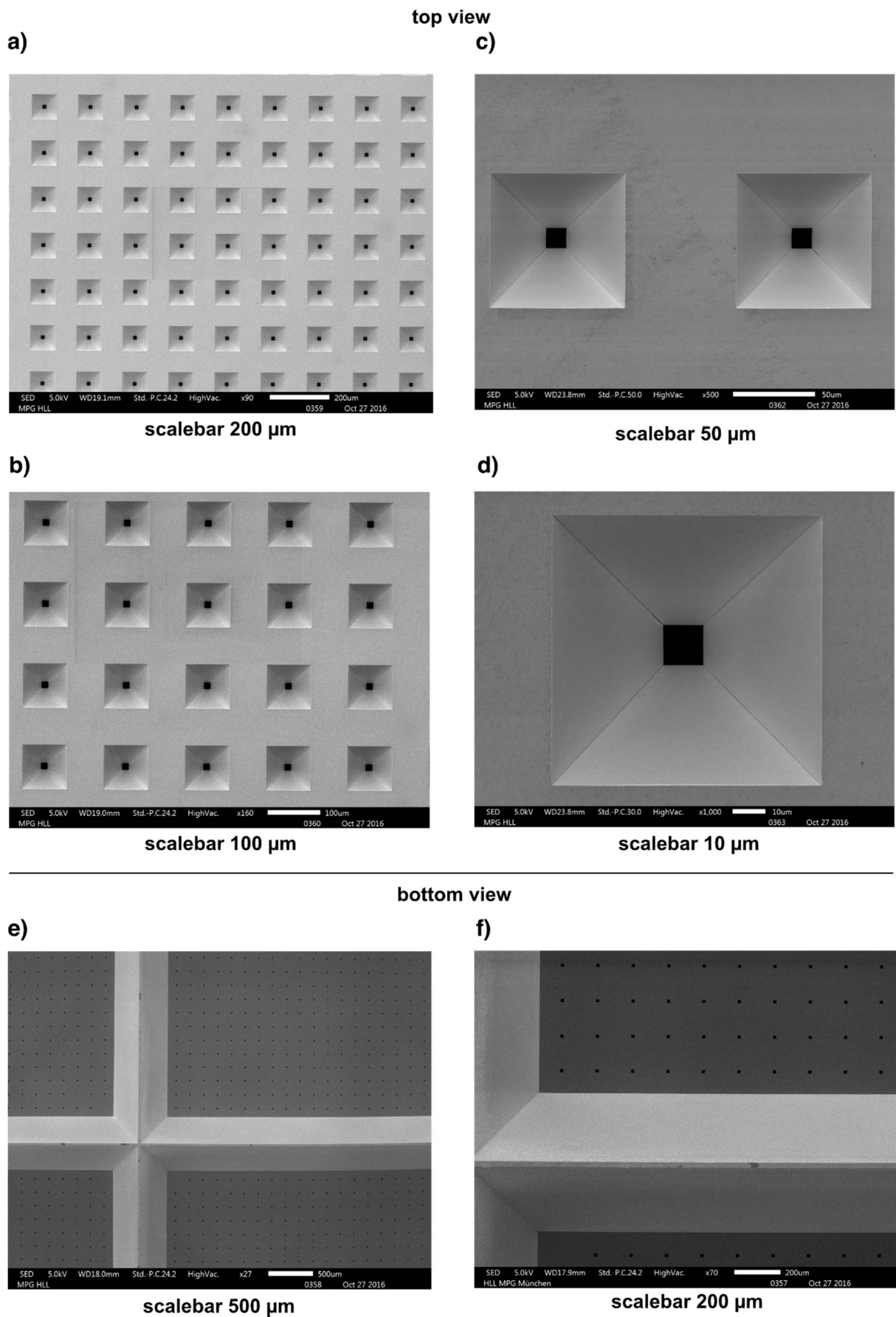
Figure S1 SEM images of the HARE chip at different magnifications.
