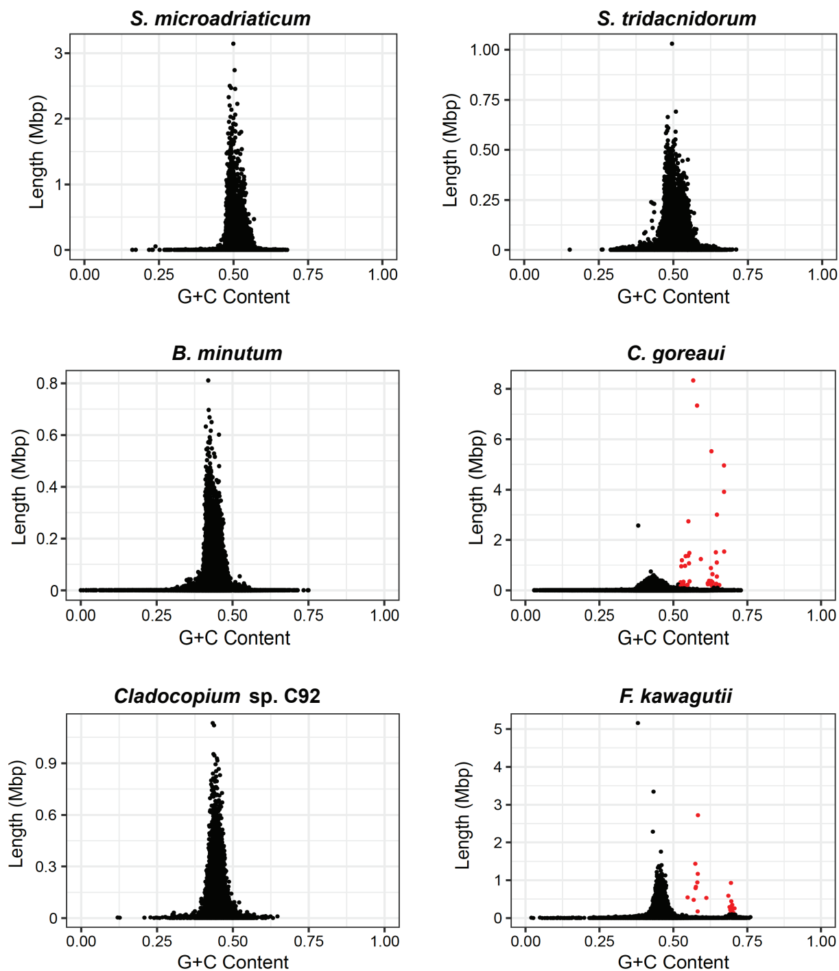
Fig. S2. Distribution of G+C percentage assembled genome scaffolds relative to scaffold length, shown for each of the six Symbiodiniaceae genomes analyzed in this study. Data points representing scaffolds that were identified as putative contaminants are highlighted in red.
