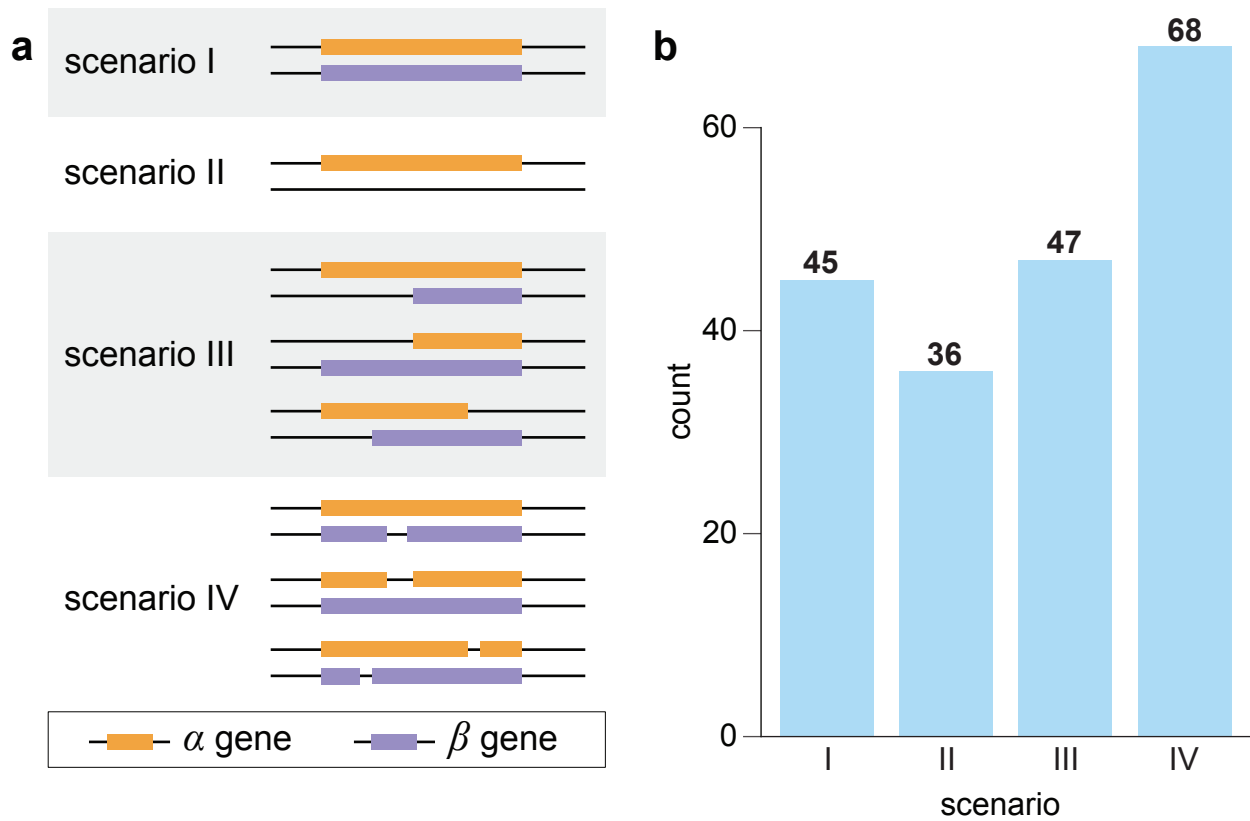
Fig. S4. Structural differences between \alpha and \beta genes. (a) Four scenarios into which the structural differences are broadly categorized. (b) Among collinear syntenic blocks shared by S. tridacnidorum and Cladocopium C92, the number of implicated \alpha genes that fall into each of the four scenarios (relative to the corresponding \beta genes) is shown.
