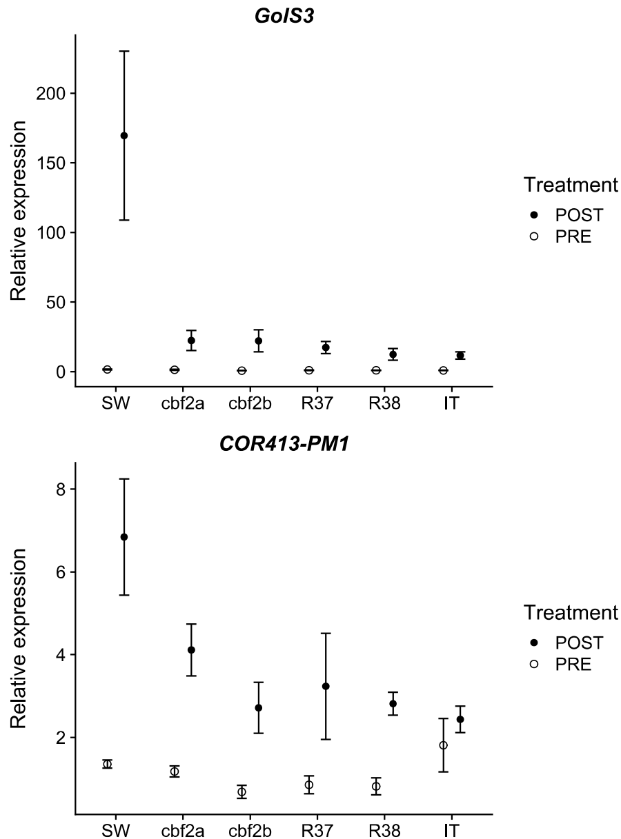
Appendix S13. Relative expression for GolS3 and COR413-PM1 quantified by RT-qPCR, normalized to expression of the housekeeping gene ACT2 . PRE and POST refer to pre-acclimation and post-acclimation tissue collections, respectively. Each biological replicate was run in triplicate for three technical replicates. Points are means of three biological replicates, and error bars are the standard error of those means. Primer sequences used are as follows: GolS3 F, 5-TGTGCCAAAGCTCCATCCGC-3; GolS3 R, 5-TGGTGTGACAAGAACCTCGCT-3; COR413-PM1 F, 5-TGCTGGCACATTCAGAGACAG-3; COR413-PM1 R, 5-CAGACGGGGAAGACGACGAGA-3; ACT2 F, 5-CTGGATCGGTGGTTCCATTC-3; ACT2 R, 5-CCTGGACCTGCCTCATCATAC-3
