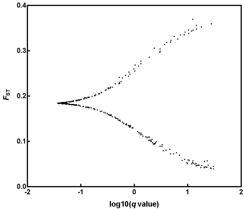
Figure S1 Neutrality tests for examining the F_{ST} distribution of microsatellite loci by the BayeScan approach.
