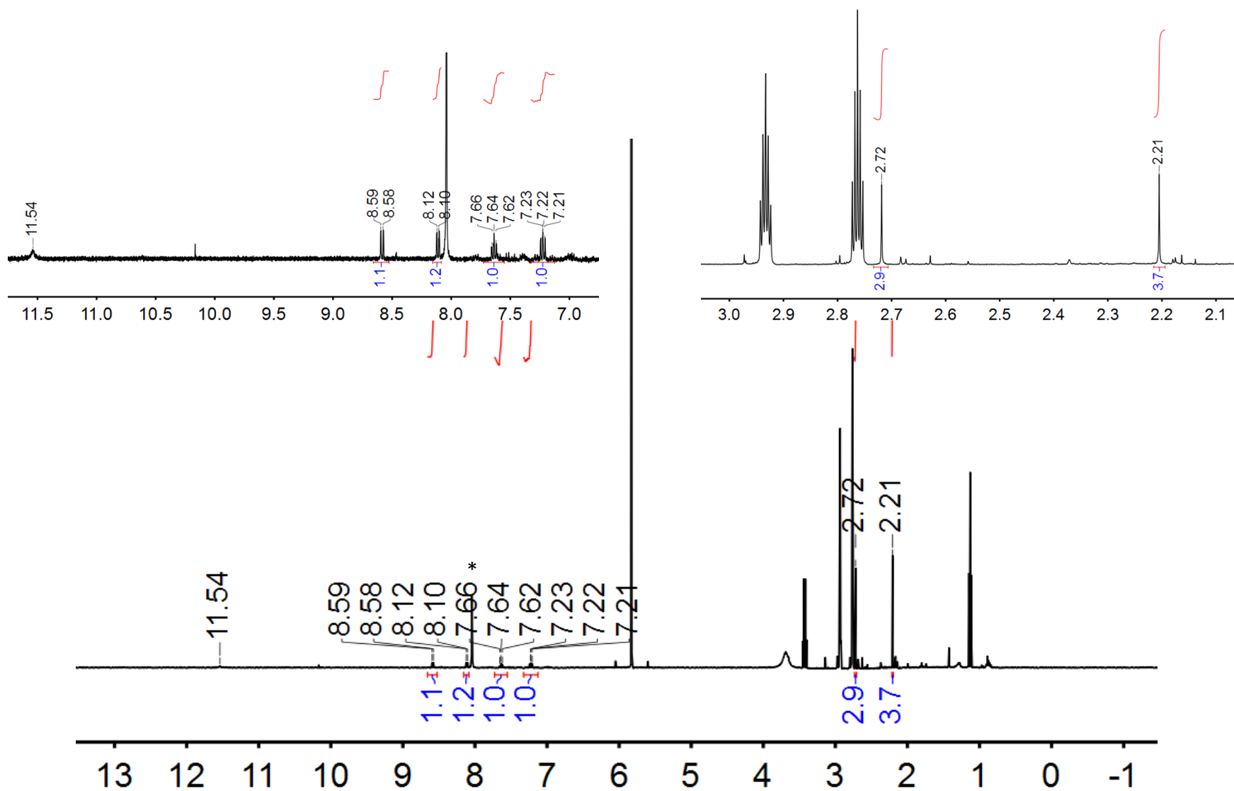
Figure S6. 1 H NMR spectrum (400 MHz) of the product N -(2-acetyl-phenyl)-acetamide, isolated from a reaction mixture of Fe III (O 2 - )(TPP) and 2,3-DMI in DMF- d 7 .
