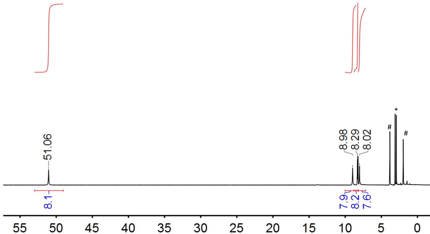
Figure S2. ^1\text{H} NMR spectrum (400 MHz) of \text{Fe}^{\text{II}}(\text{TPP}) (4 mM) in \text{DMF-}d_7 at 25 °C; * = DMF, # = THF.
