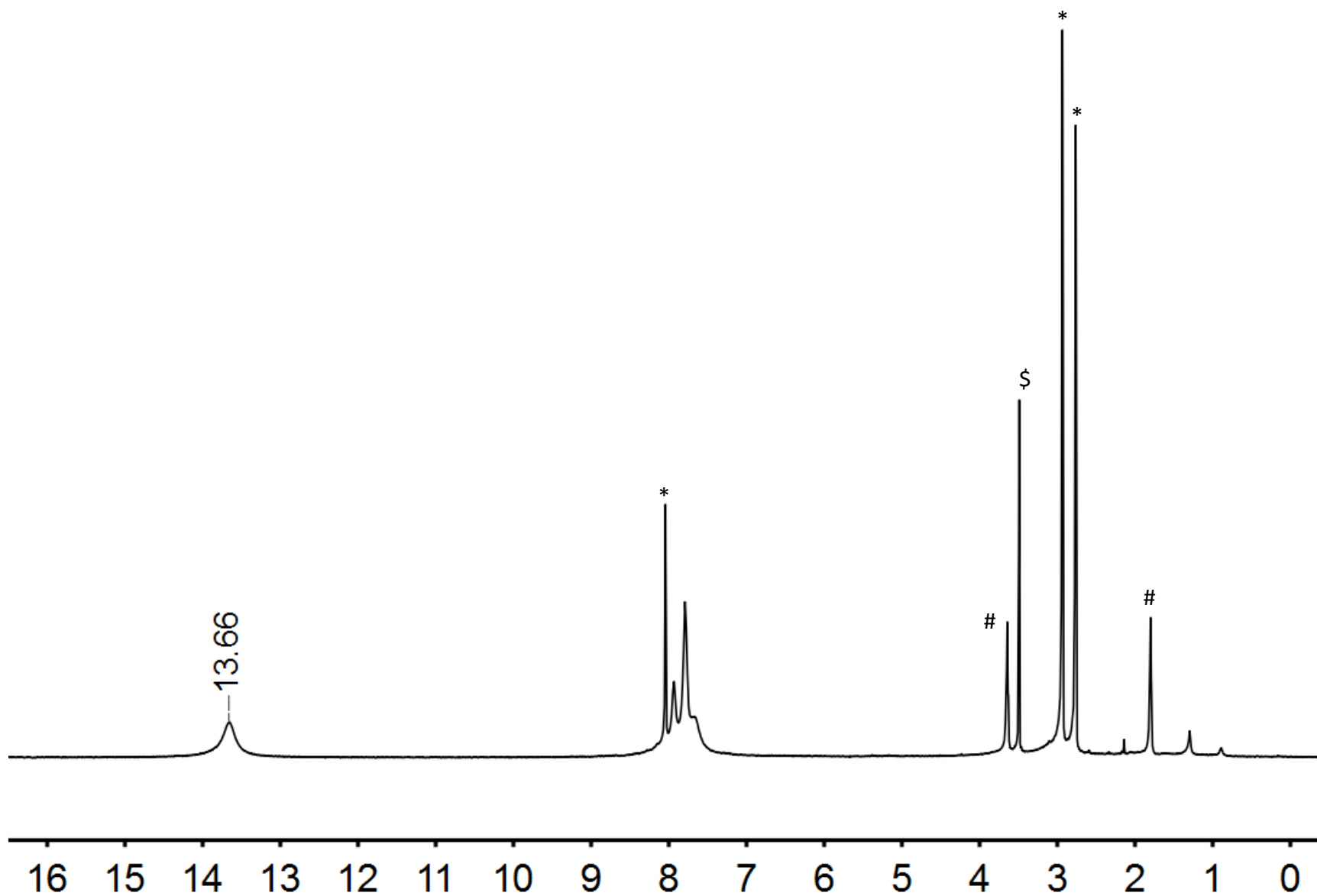
Figure S4. 1 H NMR spectrum (400 MHz) of (Fe III (TPP)) 2 (μ-O) (4 mM) in DMF- d 7 at 25 °C; * = DMF, # = THF, $ = H 2 O.
