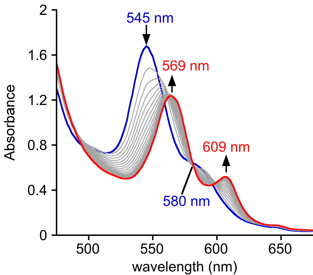
Figure S1. Time-resolved UV-vis spectral changes (0 – 120 min) observed for the self-decay of \text{Fe}^{\text{III}}(\text{O}_2^{\cdot-})(\text{TPP}) (0.6 mM) to form (\text{Fe}^{\text{III}}(\text{TPP}))_2(\mu\text{-O}) in DMF at -40\text{ }^\circ\text{C} .
