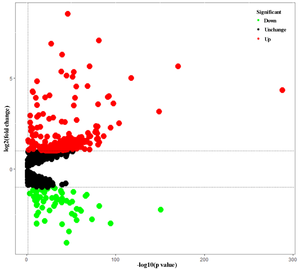
Figure S1 Differentially expressed RBPs in LUSC. Red: upregulation with \text{FC} > 2 ; green: downregulation with \text{FC} > 2 ; black: not significant.
