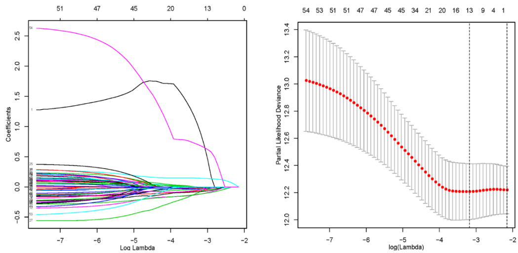
Figure S2 LASSO regression analysis for screening prognosis-related RBPs.
