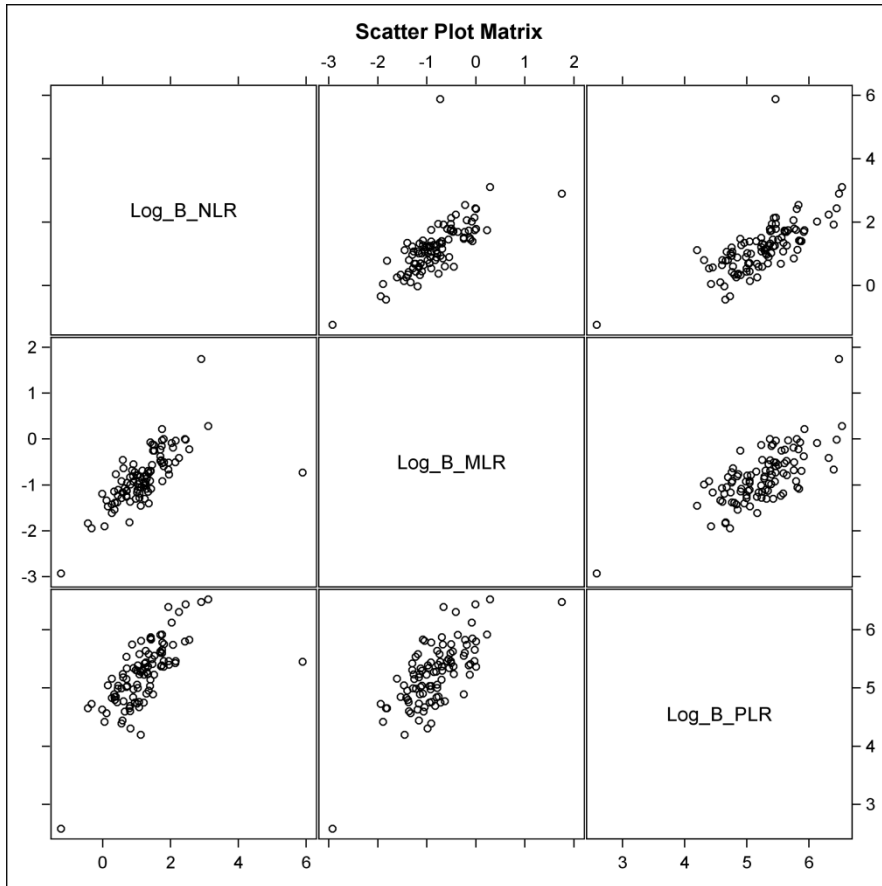
Supplemental Figure S1: Scatter matrix plot of association between NLR, MLR and PLR
