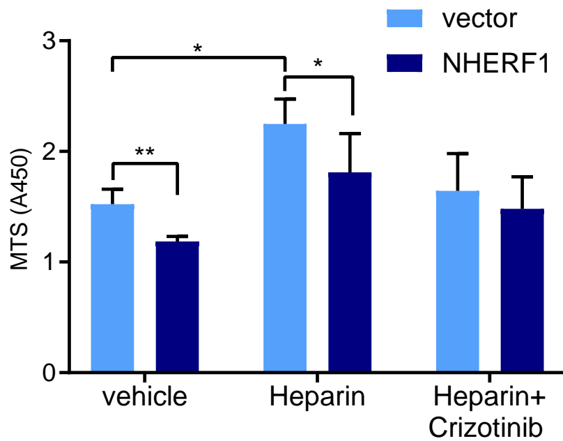
Suppl figure 1. The cell viability from MTS assays in H3122 and NHERF1 overexpressed cells in the presence of heparin (1 \mu\text{g}/\text{ml} ), or crizotinib (1 \mu\text{M} ), or both for 72 h. * p < 0.05 , ** p < 0.01 .
