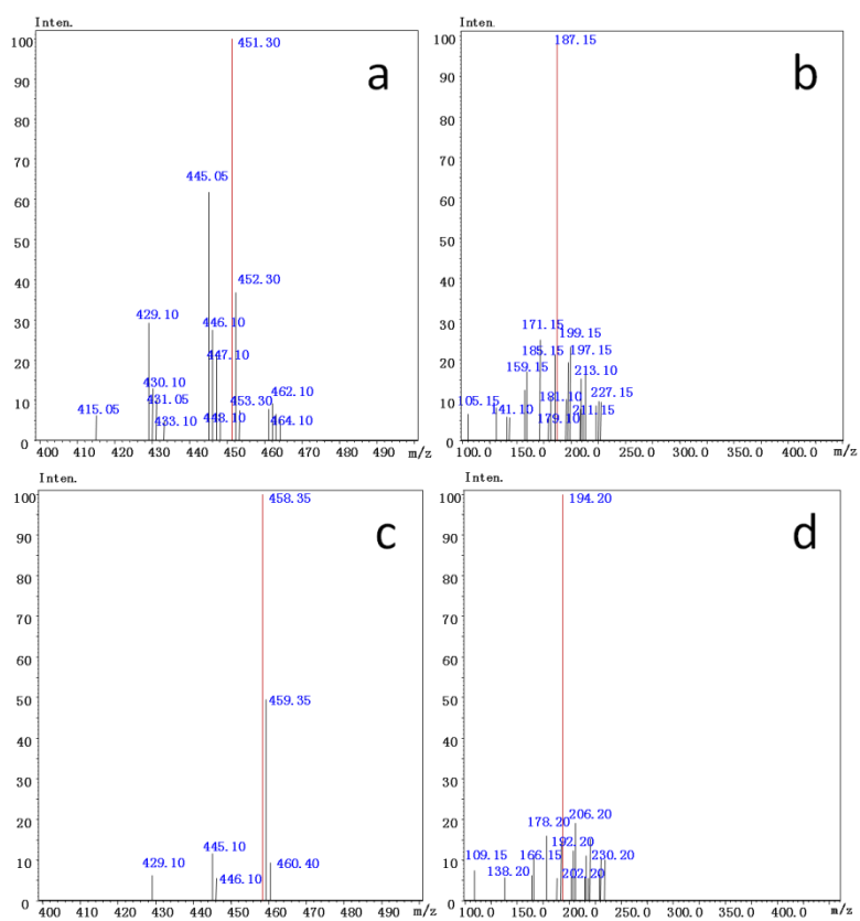
Figure S2. MS/MS spectrum of vitamin K 1 and vitamin K 1 -D 7 : (a) vitamin K 1 full scan, (b) vitamin K 1 product ion scan, (c) vitamin K 1 -D 7 full scan, (d) vitamin K 1 -D 7 product ion scan
