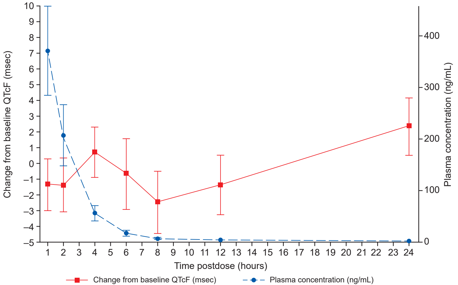
A. \Delta QTcF vs. time and evobrutinib concentration versus time, superimposed
